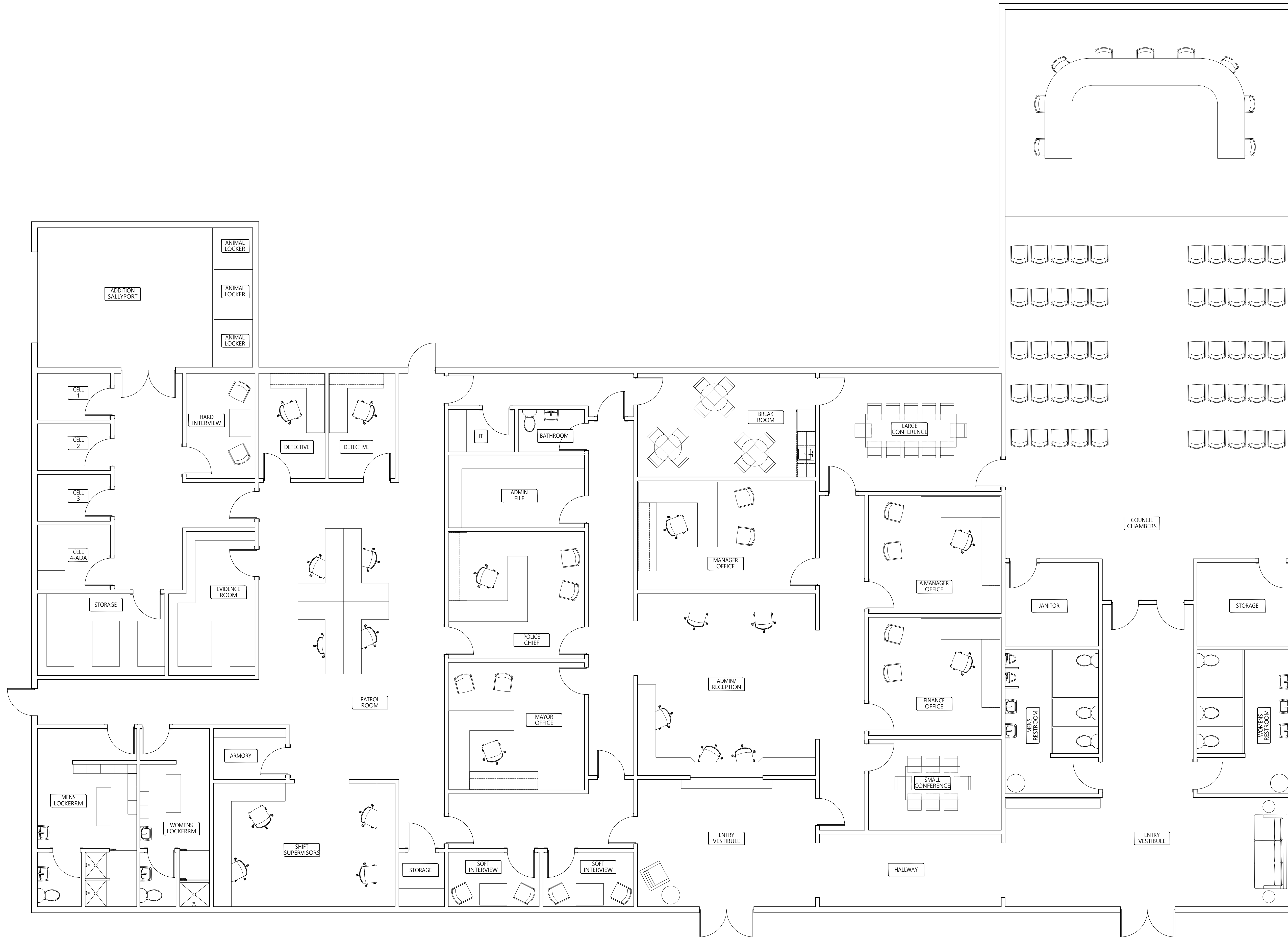
1 PROPOSED FLOORPLAN SD SCALE: 3/16" = 1'-0"
