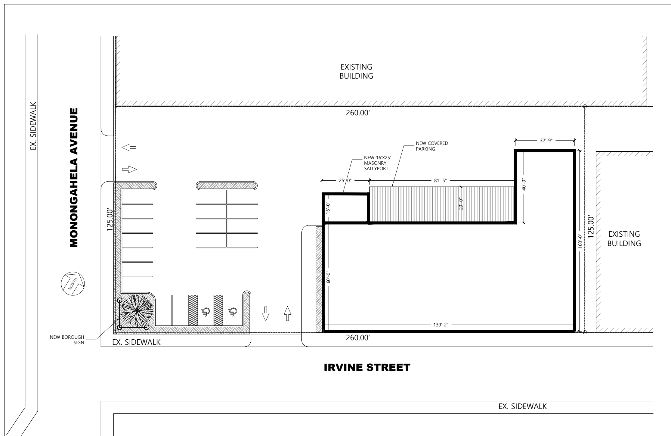
1 PROPOSED PLAN PL SCALE: 1/32" = 1'-0"
